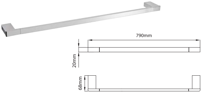
TOWEL RAIL - SINGLE (750) 122207 BRASS
