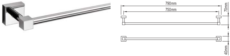
TOWEL RAIL - SINGLE 113144 BRASS
