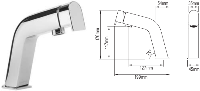
BASIN MIXER 5★ (6L/m) 105805 PADDLE FIXED
