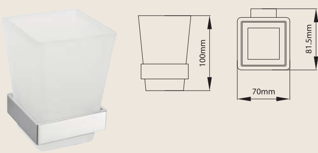
TUMBLER HOLDER 122213 BRASS
