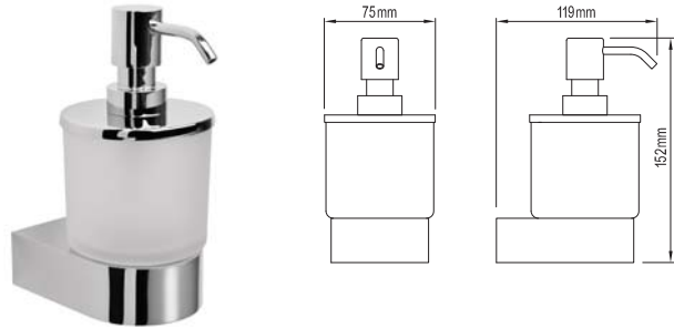
SOAP DISPENSER 113161 BRASS
