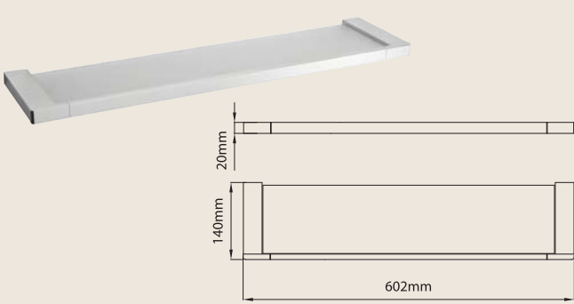
GLASS SHELF 122217 BRASS
