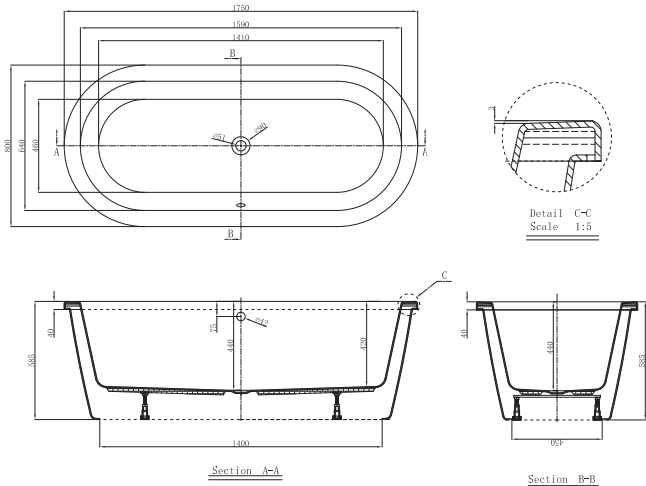
OVAL FREESTANDING BATH 114323 1750 OVAL
