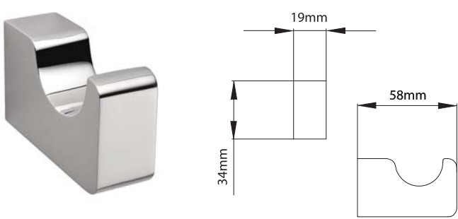
ROBE HOOK 122212 BRASS
