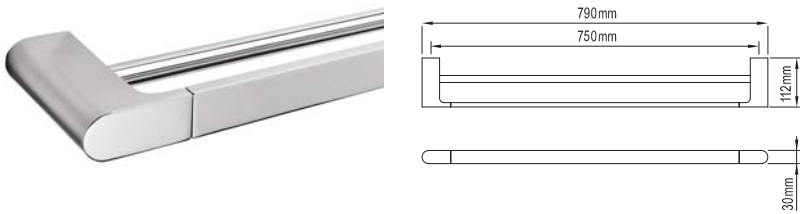
TOWEL RING 113160 BRASS
