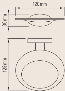
SOAP DISH 113166 BRASS
