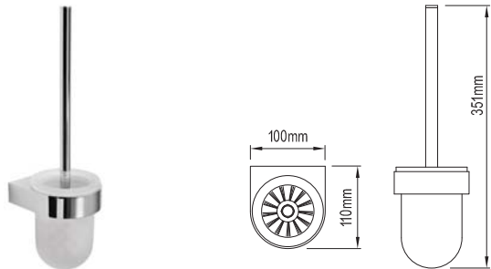
TOILET BRUSH HOLDER 113162 BRASS
