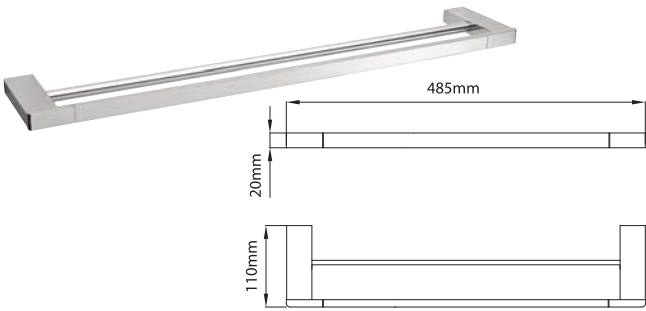
TOWEL RAIL - DOUBLE (450) 122208 BRASS
