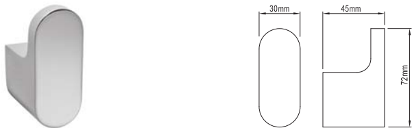
ROBE HOOK 113157 BRASS
