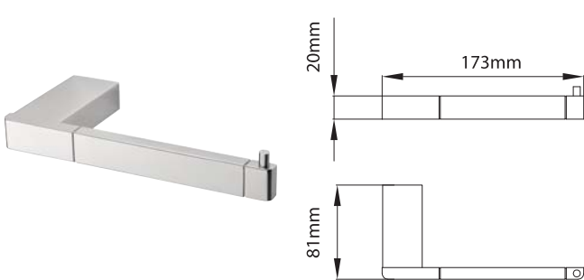
TOILET ROLL HOLDER 122211 BRASS
