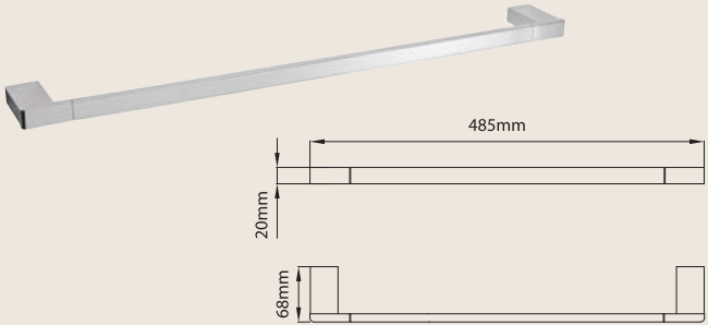
TOWEL RAIL - SINGLE (450) 122205 BRASS
