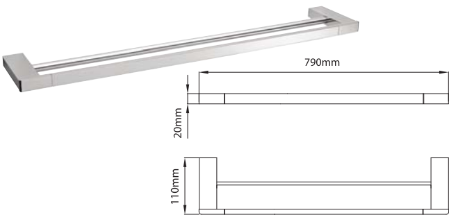
TOWEL RAIL - DOUBLE (750) 122210 BRASS
