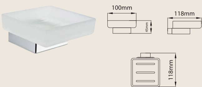
SOAP DISH 122214 BRASS
