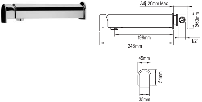
BATH SPOUT 106982 FIXED
