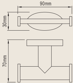
ROBE HOOK - DOUBLE 113169 BRASS
