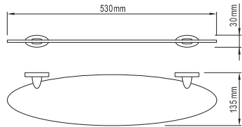
GLASS SHELF 113172 BRASS
