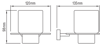
TUMBLER / TOOTHBRUSH HOLDER 113165 BRASS
