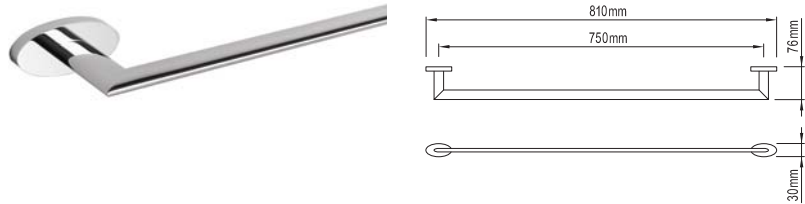
TOWEL RAIL - SINGLE 113140 BRASS
