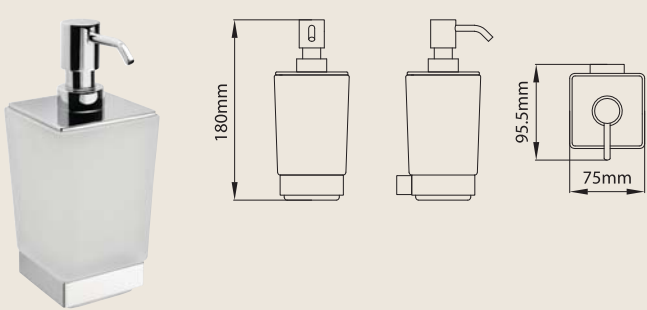
SOAP DISPENSER 122216 BRASS
