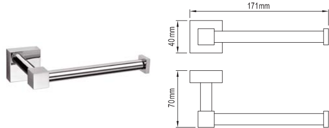
TOILET ROLL HOLDER 113146 BRASS
