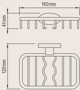
SOAP BASKET 113168 BRASS
