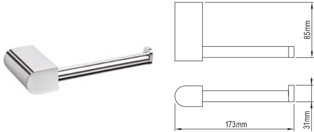
TOILET ROLL HOLDER 113156 BRASS
