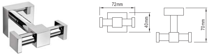
ROBE HOOK - DOUBLE 113148 BRASS
