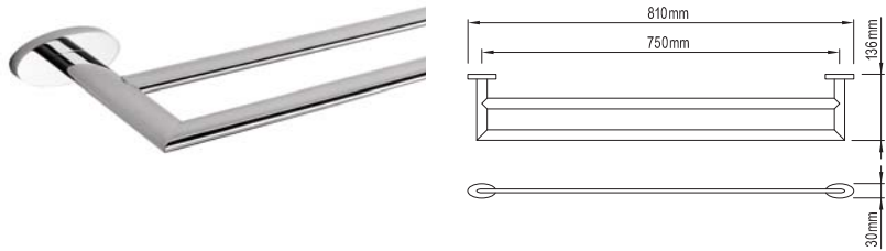
TOWEL RAIL - DOUBLE 113141 BRASS
