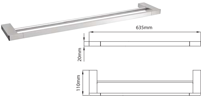
TOWEL RAIL - DOUBLE (600) 122209 BRASS
