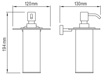
SOAP DISPENSER 113143 BRASS
