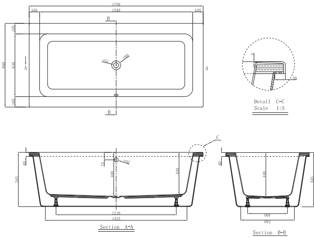
RECTANGULAR FREESTANDING BATH 114322 1750 RECT
