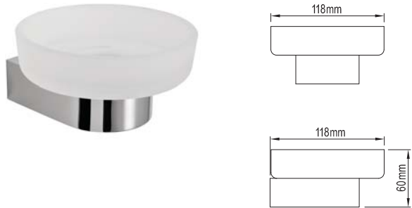
SOAP DISH 113159 BRASS
