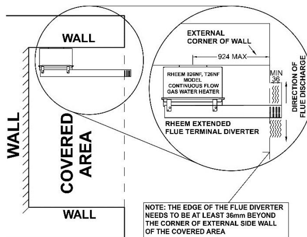
826NF or T26NF with an Extended Flue Terminal Diverter installed in compliance with AS/NZS 5601.1
