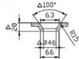
OUTLET HOLE DETAIL
