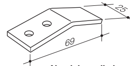
Aluminium clip bracket Code No.813734
